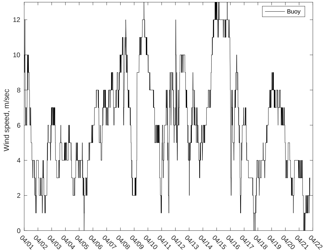
NDBC 41013 vs AUSWAV Winds: 7 to 10 day forecast
