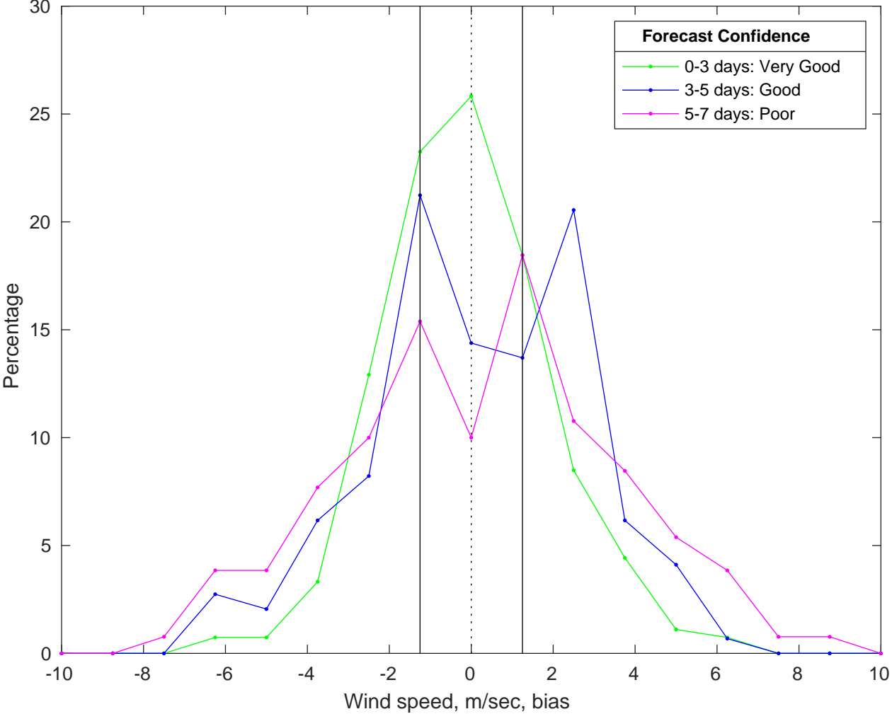
NDBC 41013 vs AUSWAV Winds Bias Histogram: 21-Apr-2025
