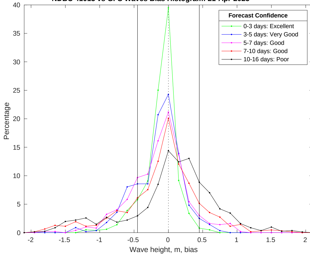
NDBC 41013 vs GFS Waves Bias Histogram: 21-Apr-2025
