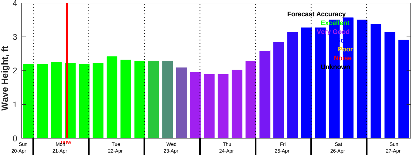
AUSWAV Wave Forecast for NDBC 41013 from 20-Apr-2025 19:00:00 to 27-Apr-2025 19:00:00
