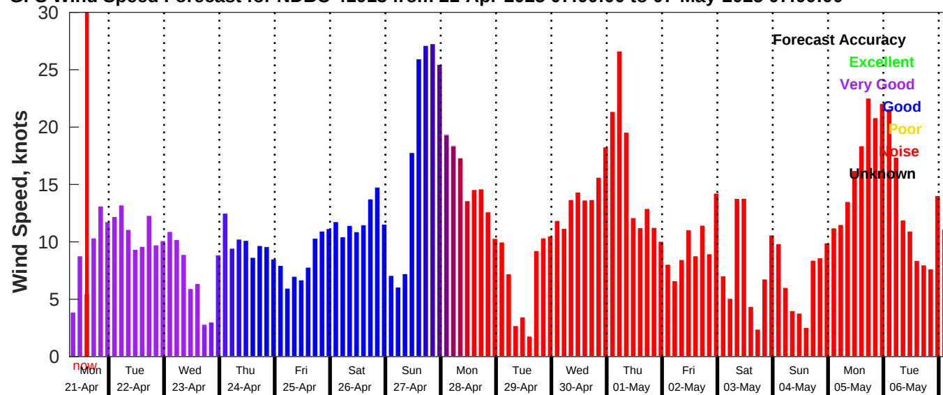
GFS Wind Speed Forecast for NDBC 41013 from 21-Apr-2025 07:00:00 to 07-May-2025 07:00:00
