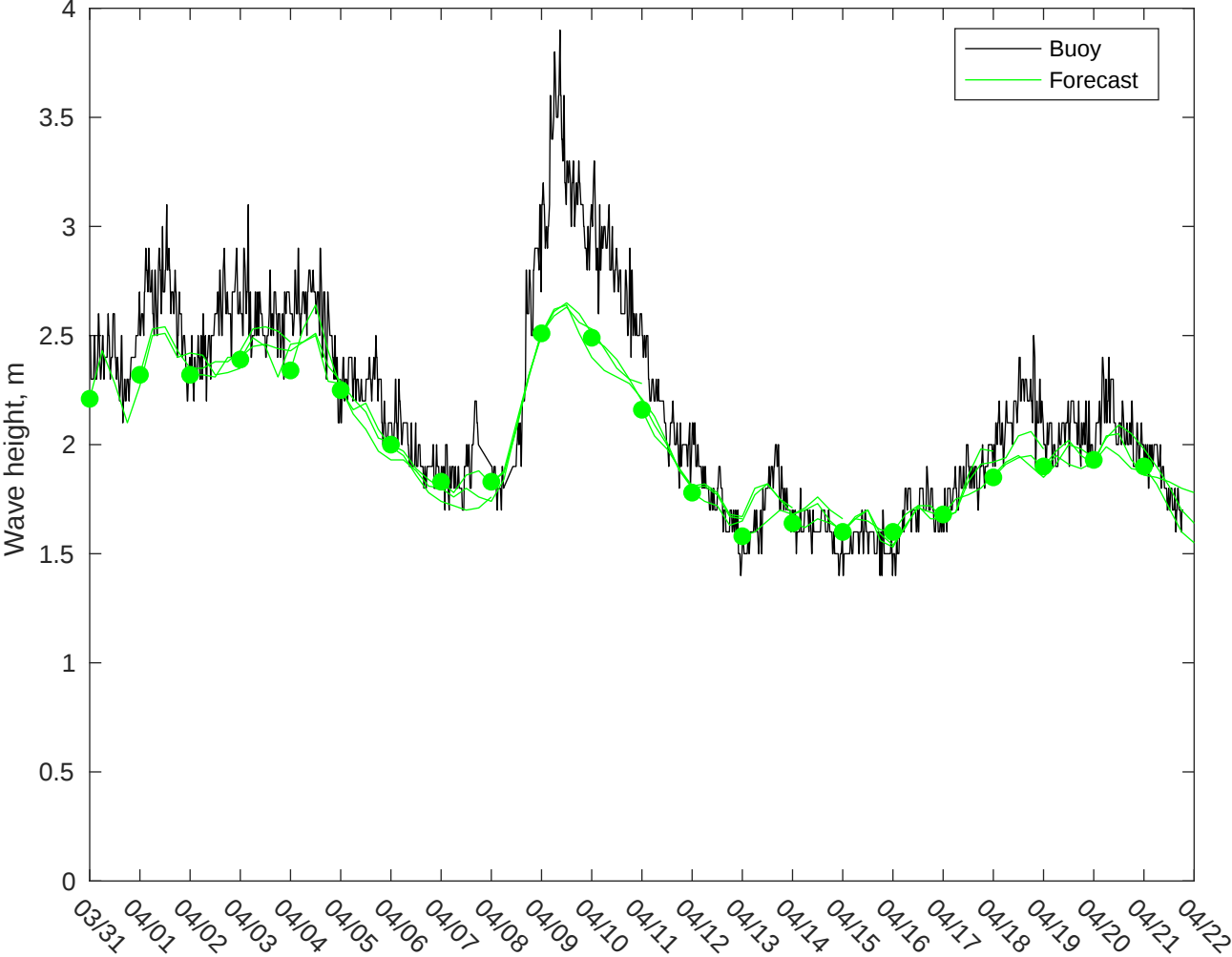
NDBC 41040 vs AUSWAV Waves: 0 to 3 day forecast
