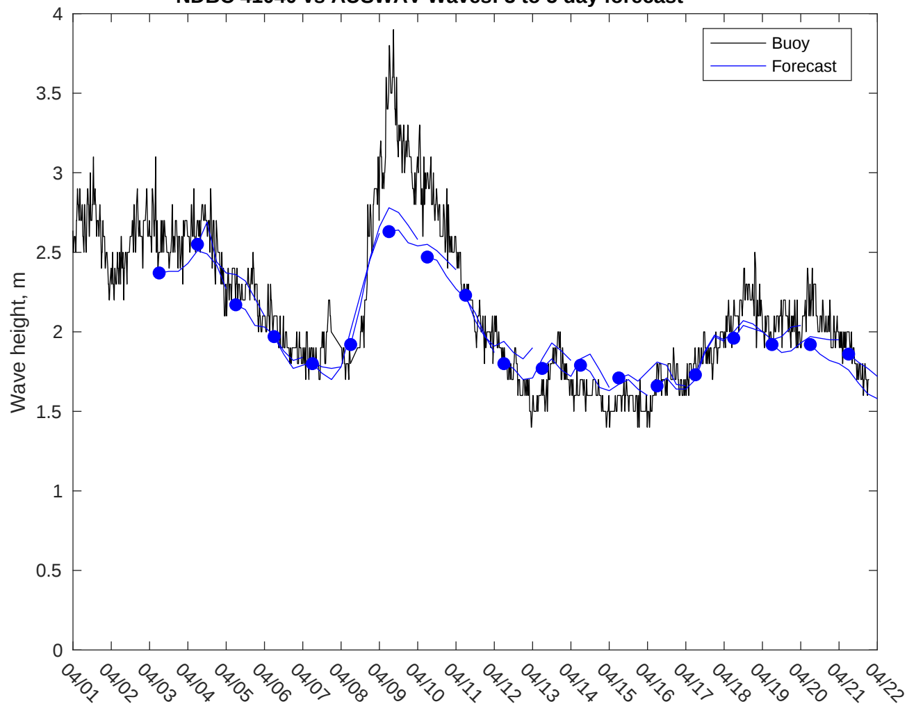
NDBC 41040 vs AUSWAV Waves: 3 to 5 day forecast
