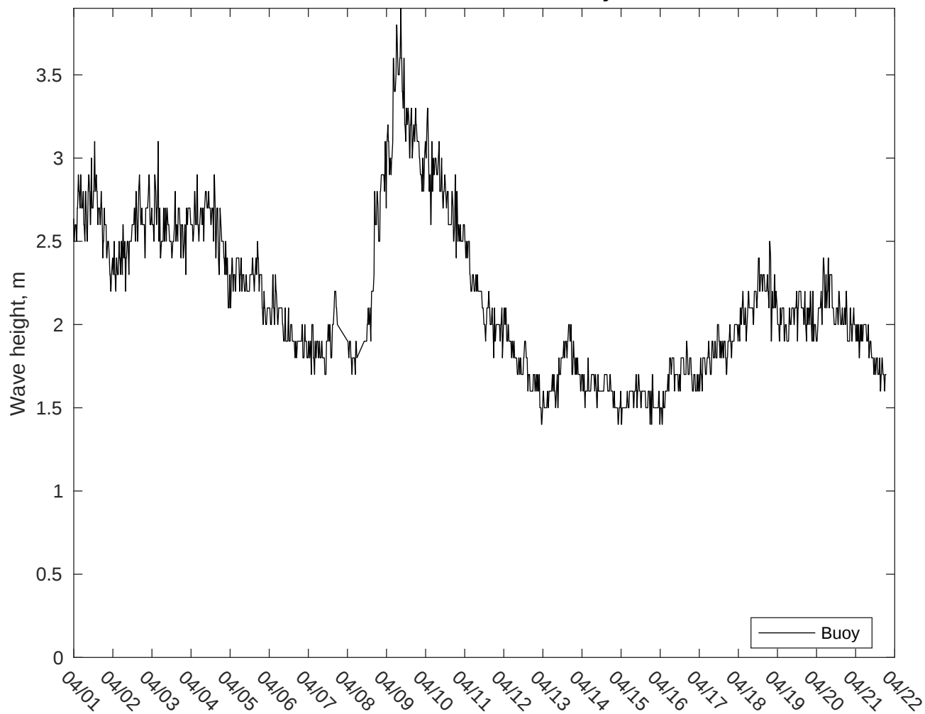
NDBC 41040 vs AUSWAV Waves: 7 to 10 day forecast
