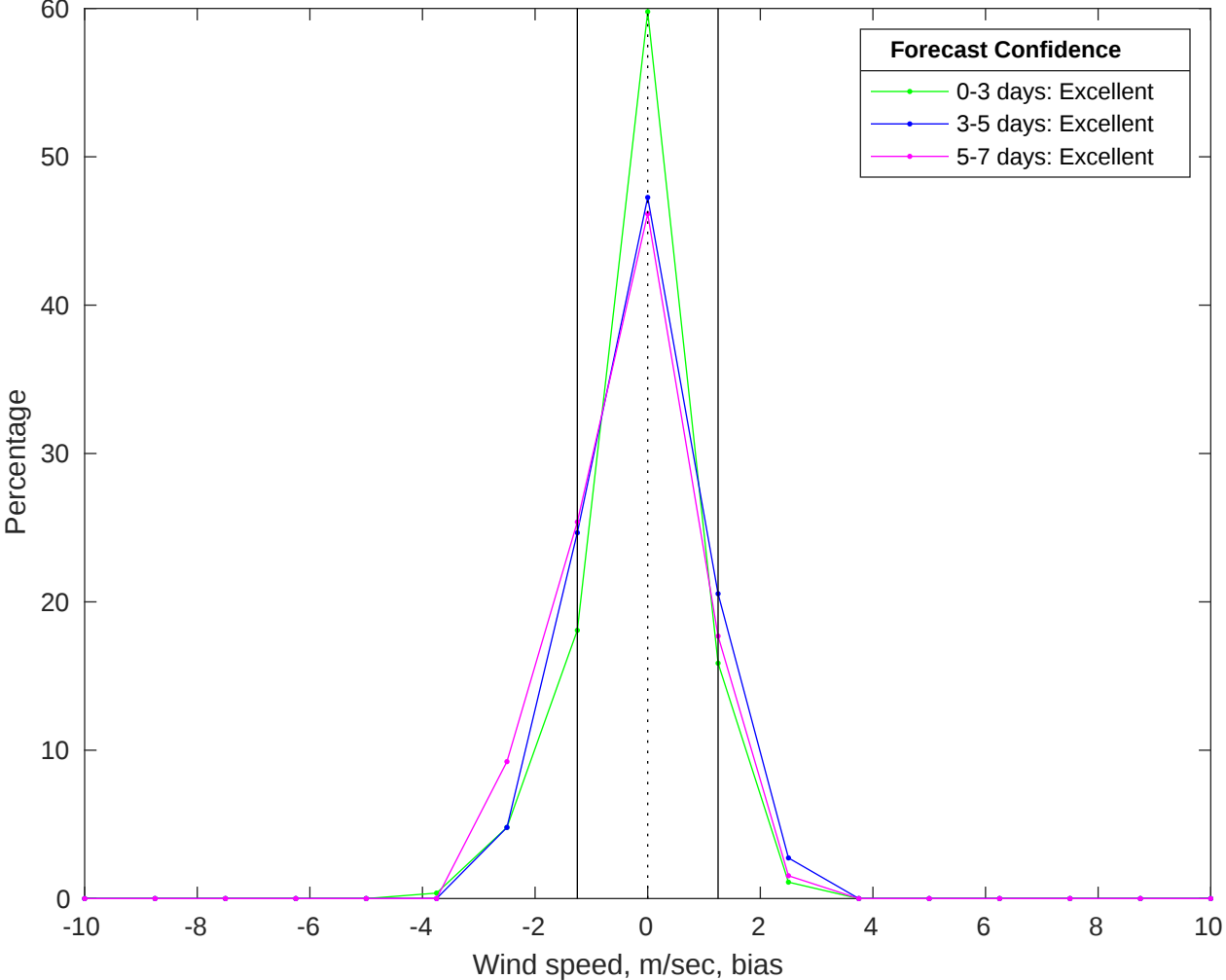
NDBC 41040 vs AUSWAV Winds Bias Histogram: 21-Apr-2025
