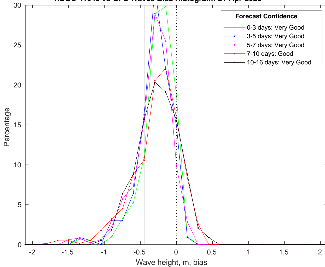
NDBC 41040 vs GFS Waves Bias Histogram: 21-Apr-2025
