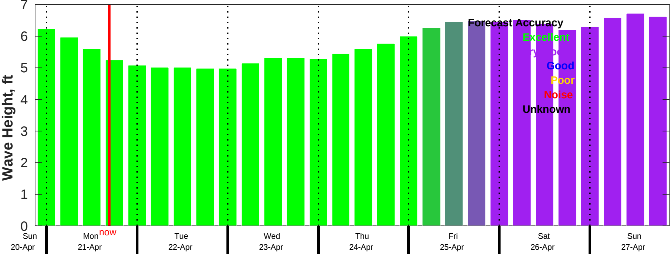
AUSWAV Wave Forecast for NDBC 41040 from 20-Apr-2025 21:00:00 to 27-Apr-2025 21:00:00
