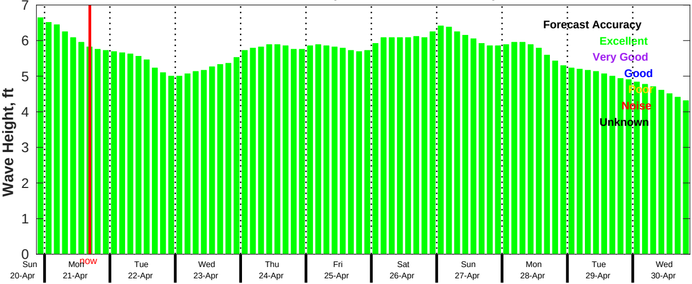
CMEMS Wave Forecast for NDBC 41040 from 20-Apr-2025 21:00:00 to 30-Apr-2025 21:00:00
