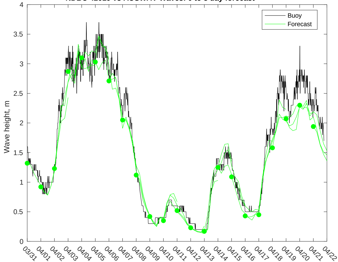
NDBC 42019 vs AUSWAV Waves: 0 to 3 day forecast
