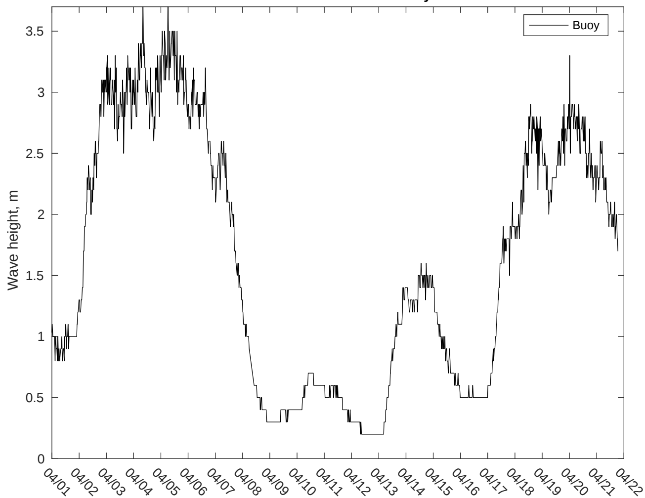
NDBC 42019 vs AUSWAV Waves: 10 to 16 day forecast
