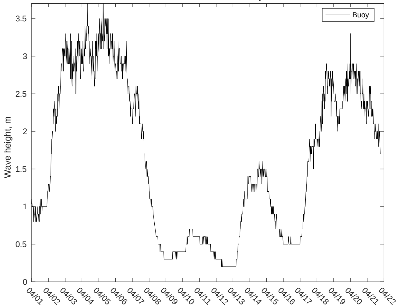
NDBC 42019 vs AUSWAV Waves: 7 to 10 day forecast
