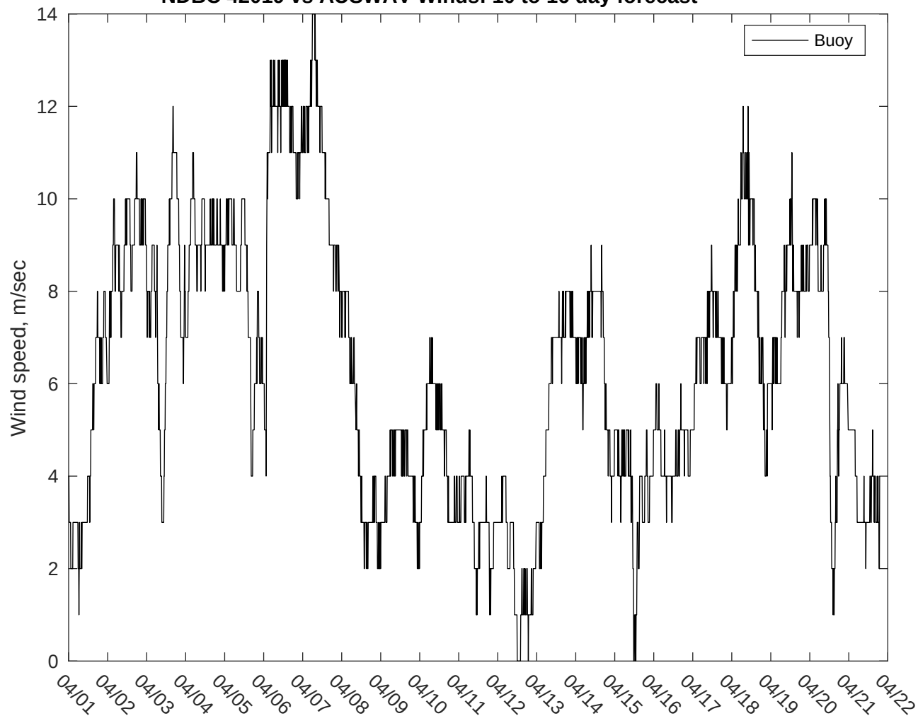
NDBC 42019 vs AUSWAV Winds: 10 to 16 day forecast
