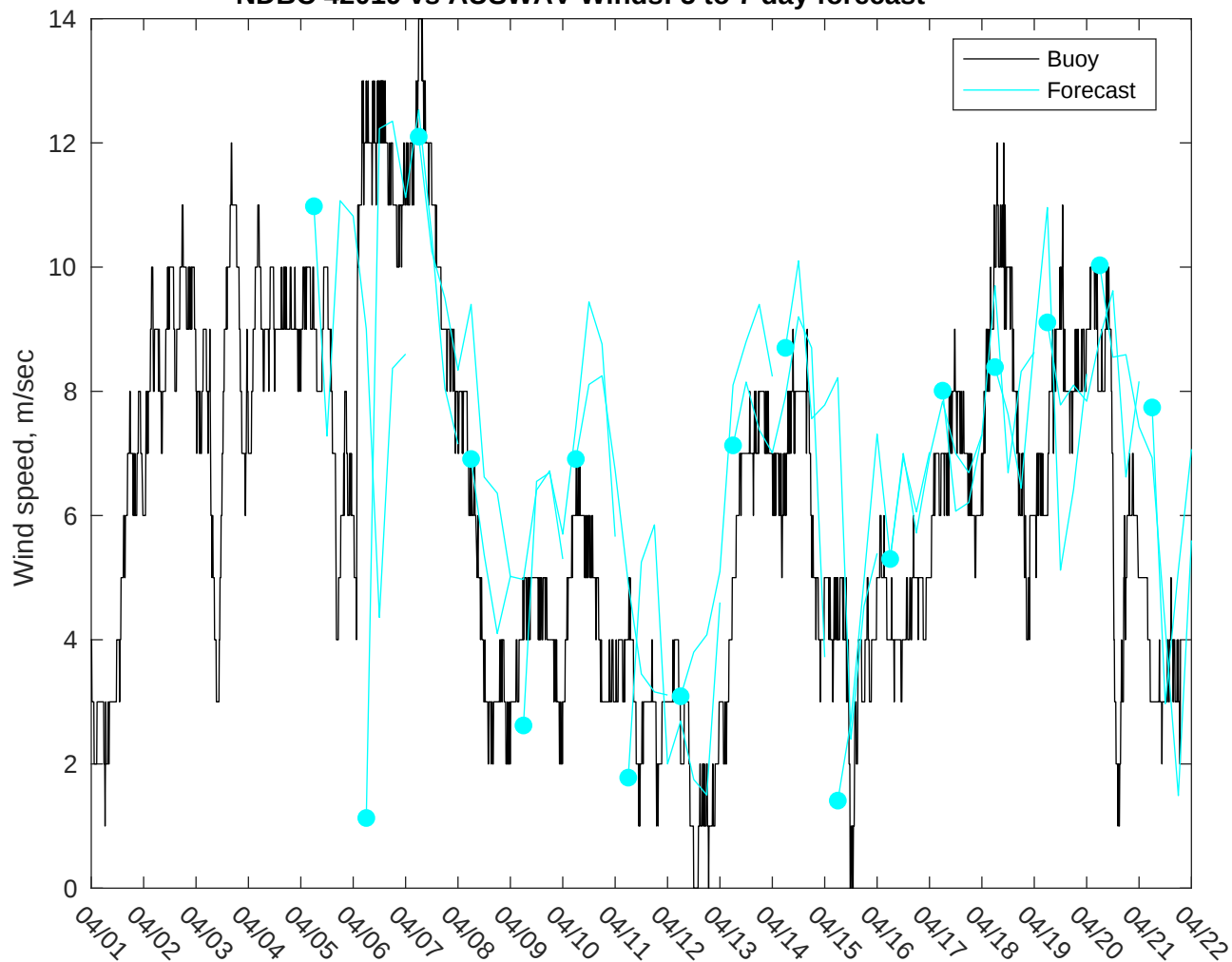
NDBC 42019 vs AUSWAV Winds: 5 to 7 day forecast
