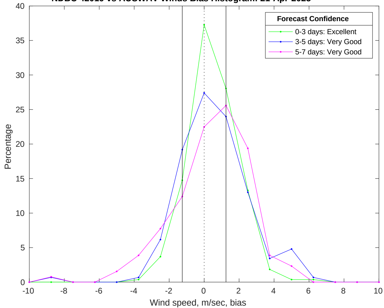
NDBC 42019 vs AUSWAV Winds Bias Histogram: 21-Apr-2025
