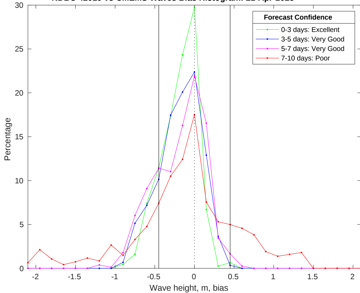
NDBC 42019 vs CMEMS Waves Bias Histogram: 21-Apr-2025
