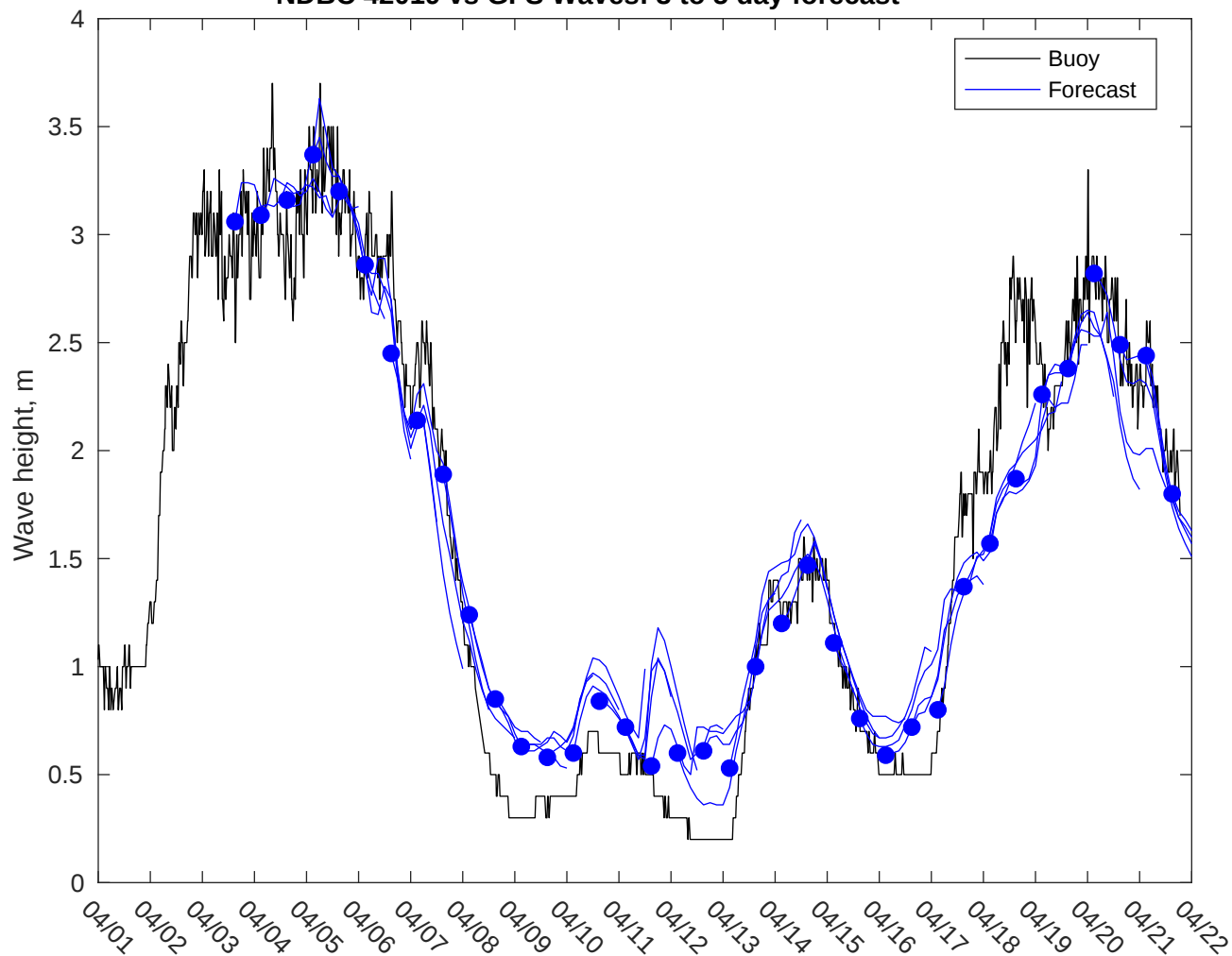
NDBC 42019 vs GFS Waves: 3 to 5 day forecast
