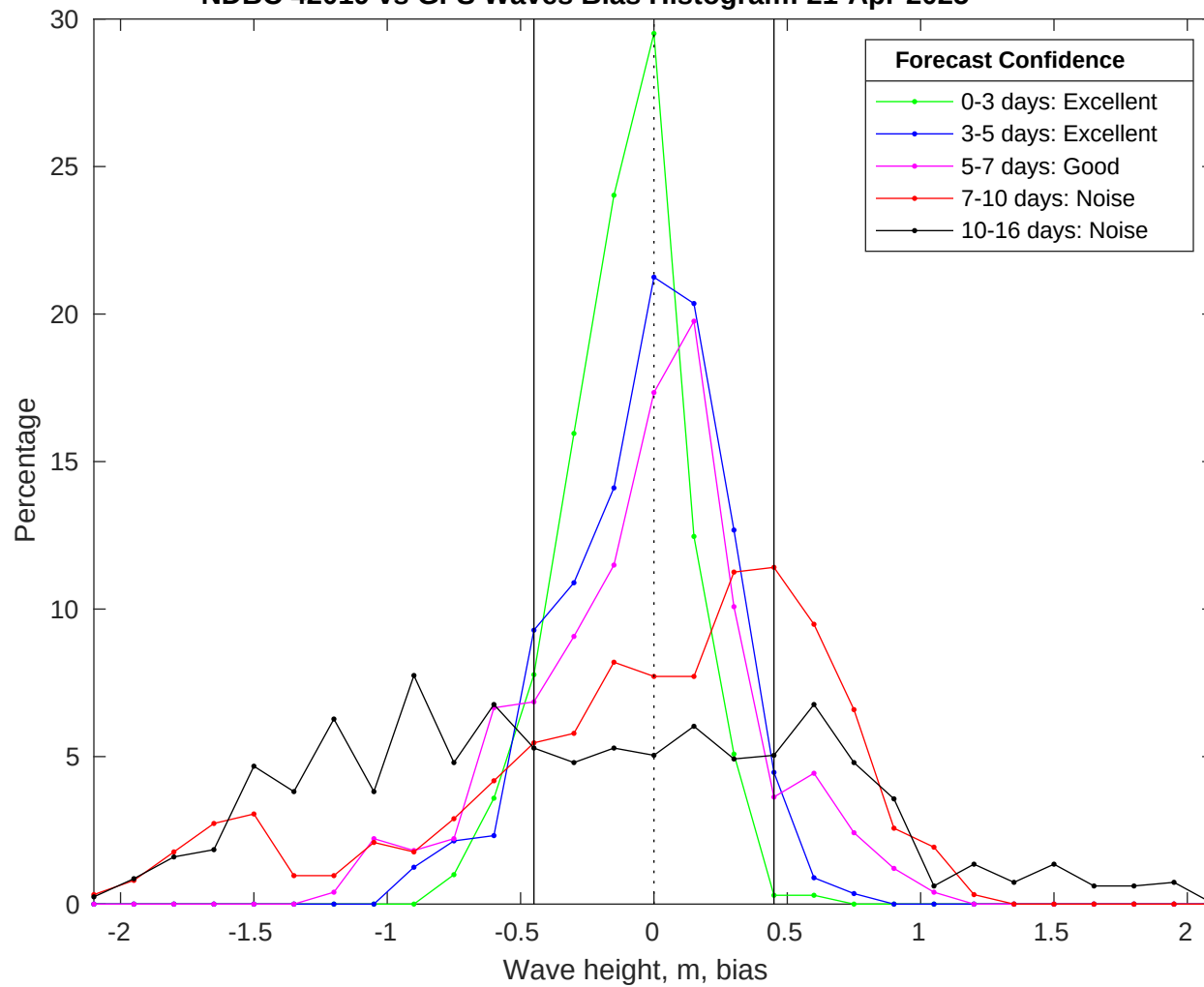
NDBC 42019 vs GFS Waves Bias Histogram: 21-Apr-2025
