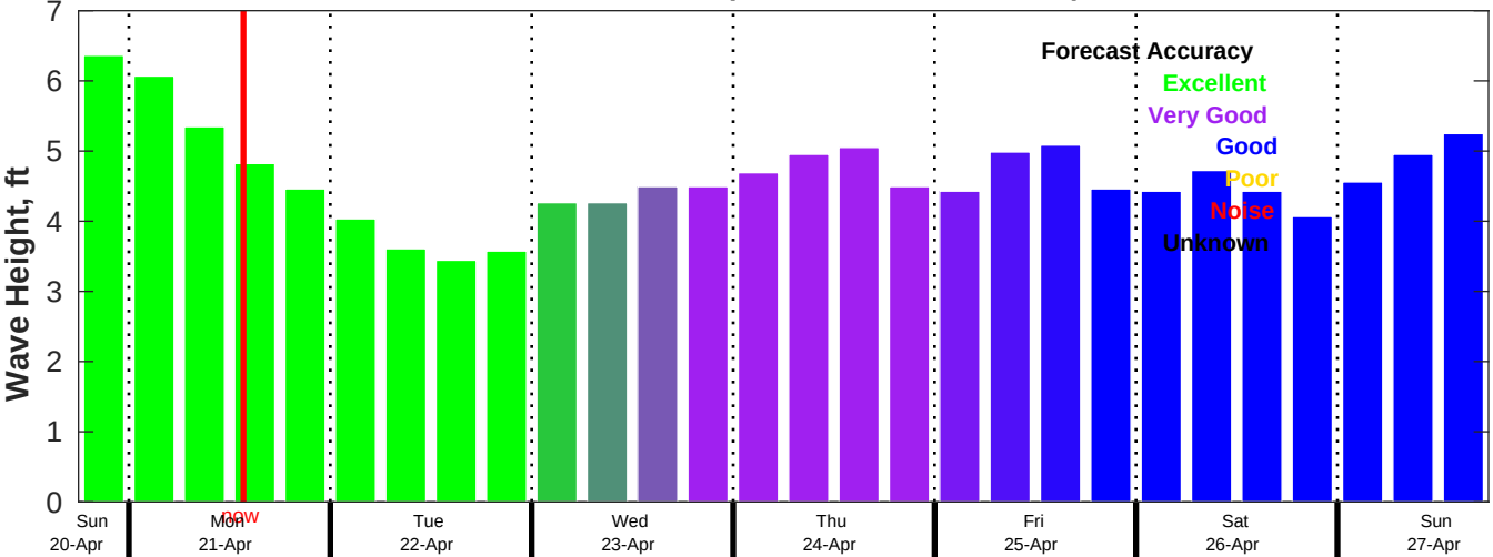
AUSWAV Wave Forecast for NDBC 42019 from 20-Apr-2025 18:00:00 to 27-Apr-2025 18:00:00
