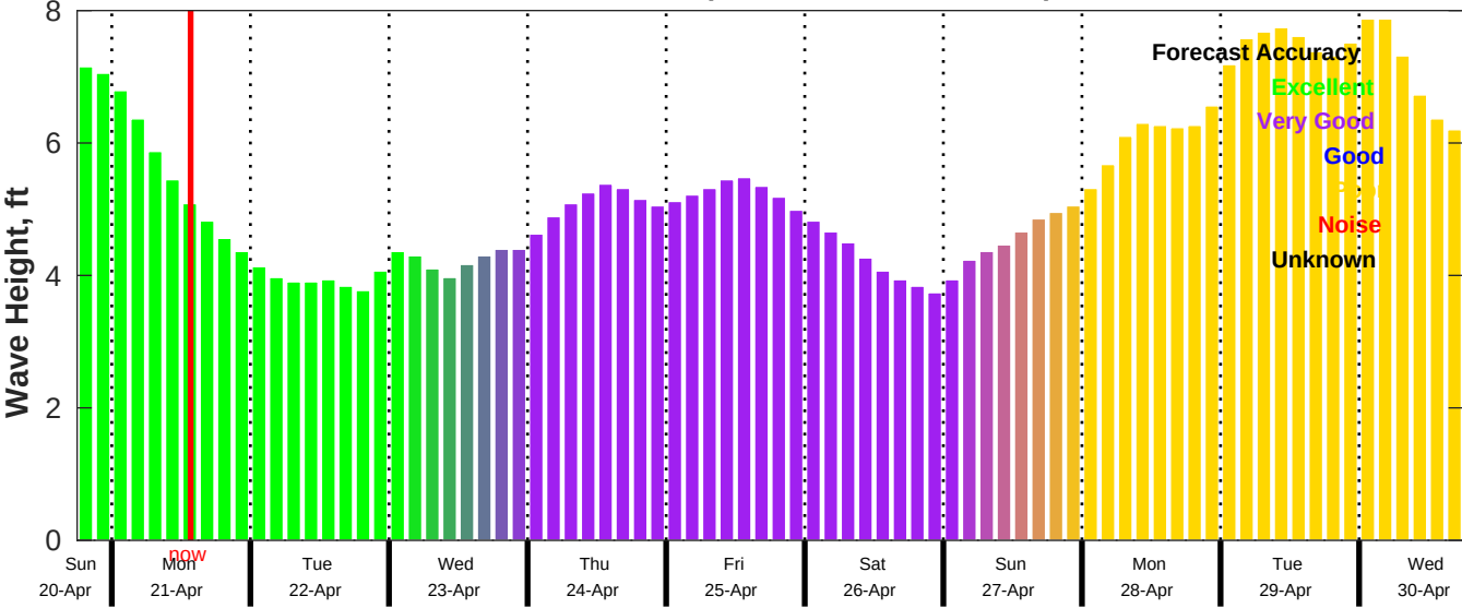
CMEMS Wave Forecast for NDBC 42019 from 20-Apr-2025 18:00:00 to 30-Apr-2025 18:00:00
