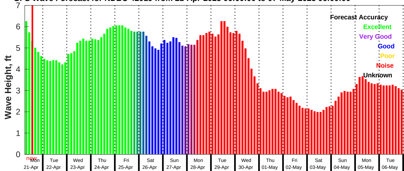
GFS Wave Forecast for NDBC 42019 from 21-Apr-2025 06:00:00 to 07-May-2025 06:00:00
