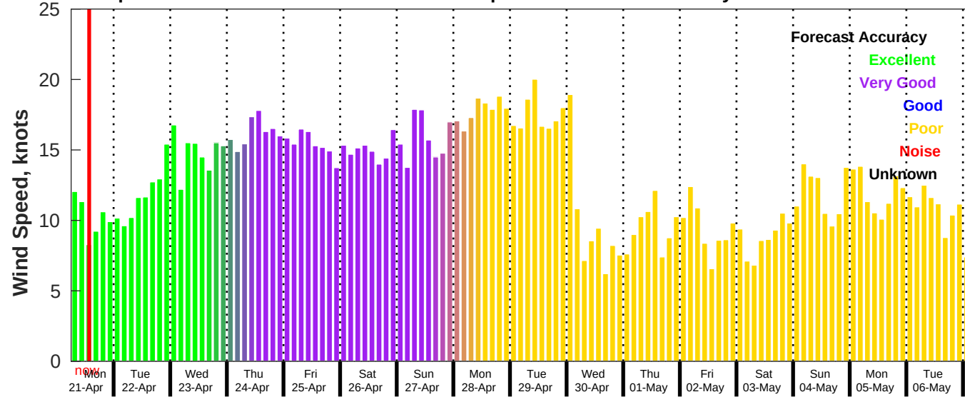
GFS Wind Speed Forecast for NDBC 42019 from 21-Apr-2025 06:00:00 to 07-May-2025 06:00:00
