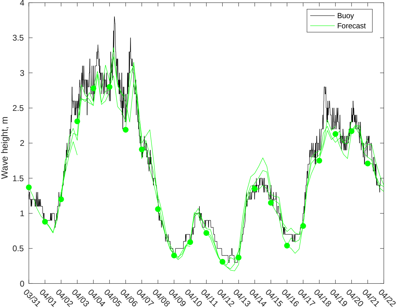
NDBC 42020 vs AUSWAV Waves: 0 to 3 day forecast
