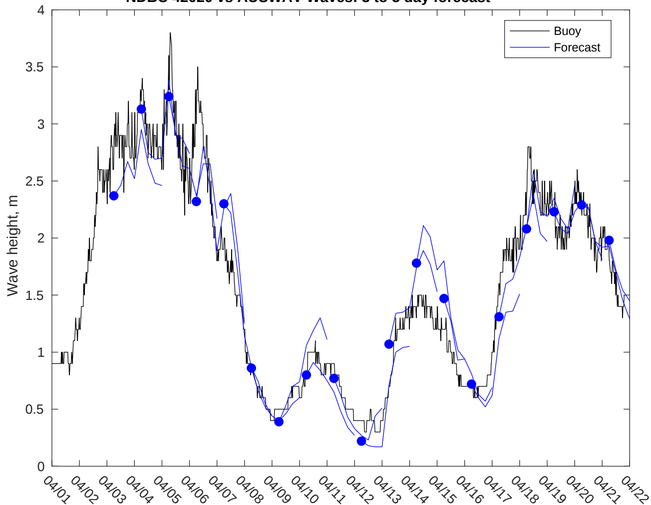
NDBC 42020 vs AUSWAV Waves: 3 to 5 day forecast
