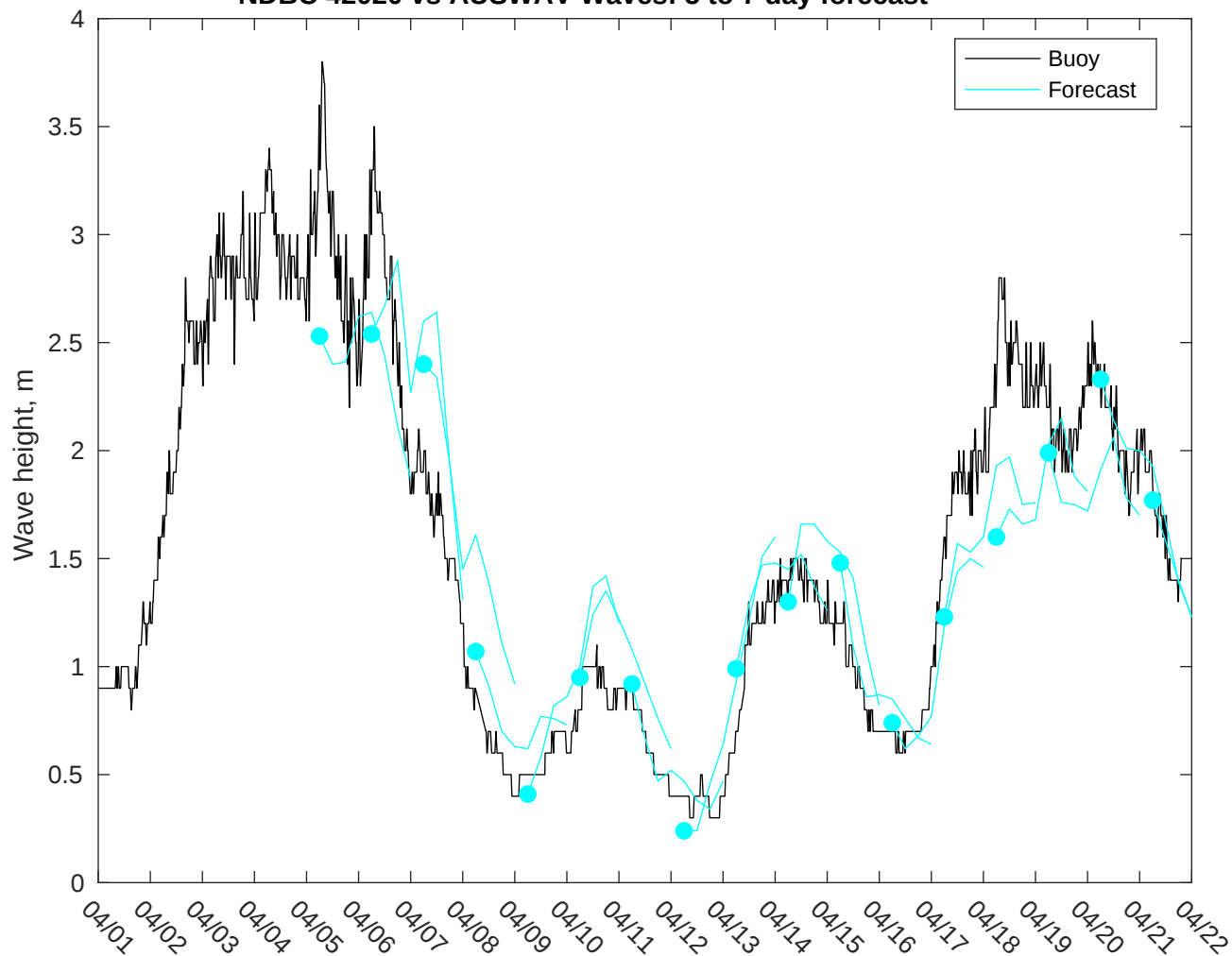
NDBC 42020 vs AUSWAV Waves: 5 to 7 day forecast
