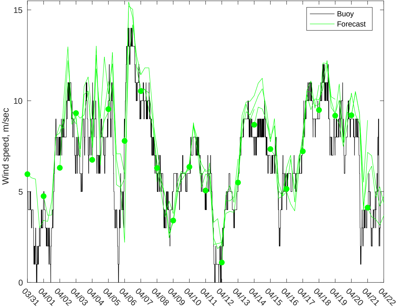
NDBC 42020 vs AUSWAV Winds: 0 to 3 day forecast
