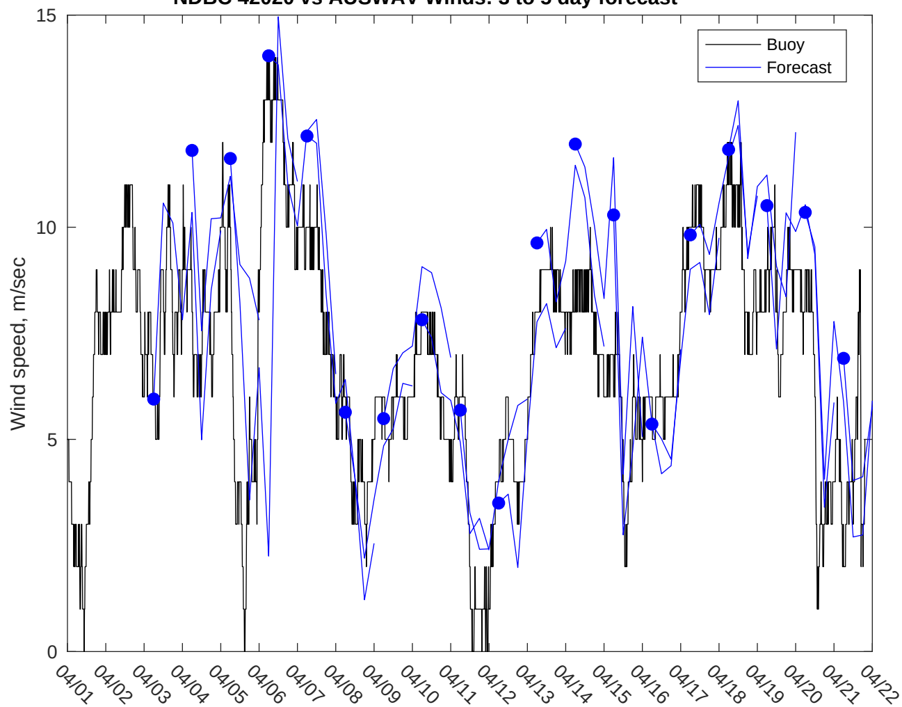
NDBC 42020 vs AUSWAV Winds: 3 to 5 day forecast
