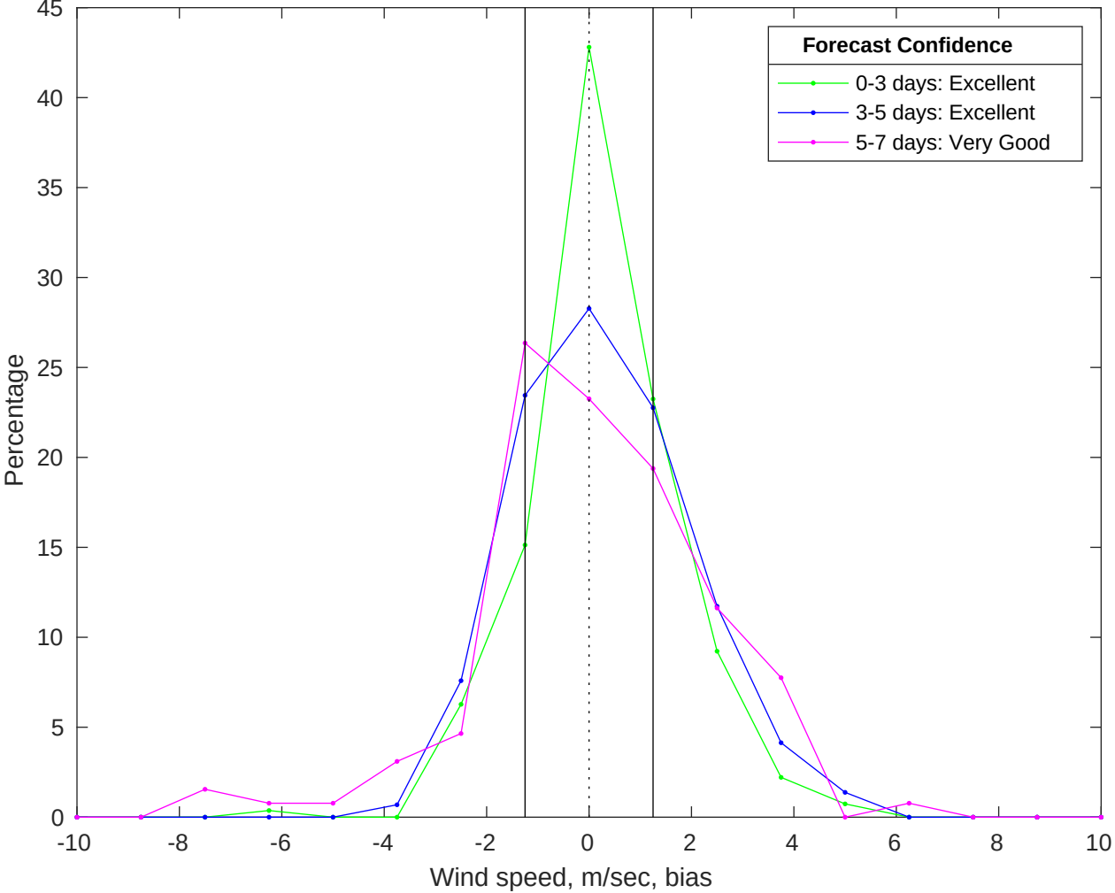
NDBC 42020 vs AUSWAV Winds Bias Histogram: 21-Apr-2025
