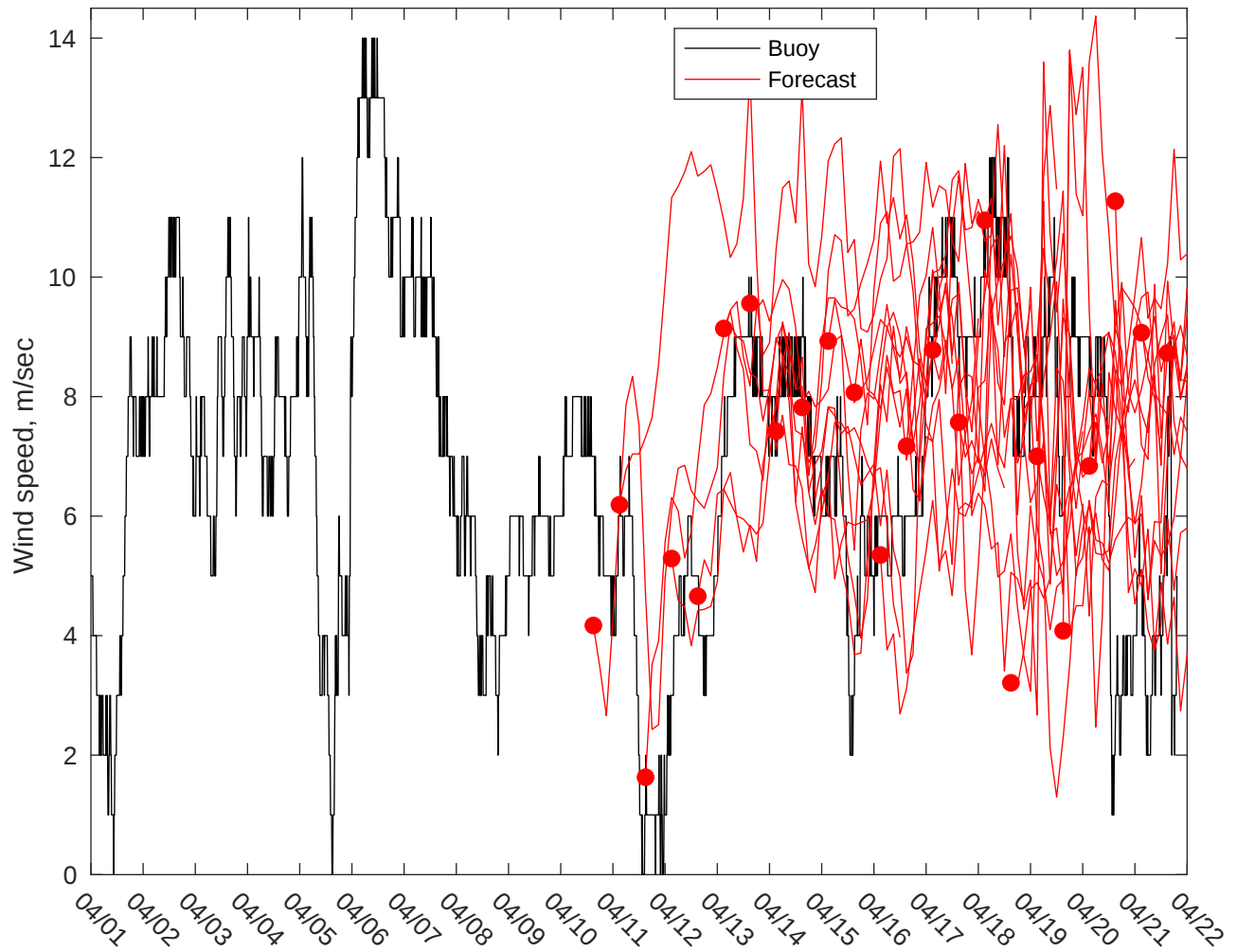
NDBC 42020 vs GFS Winds: 10 to 16 day forecast
