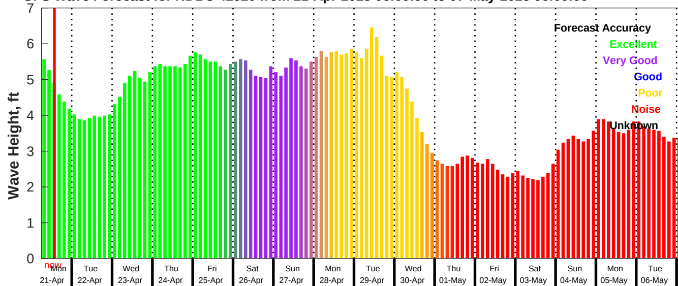
GFS Wave Forecast for NDBC 42020 from 21-Apr-2025 06:00:00 to 07-May-2025 06:00:00
