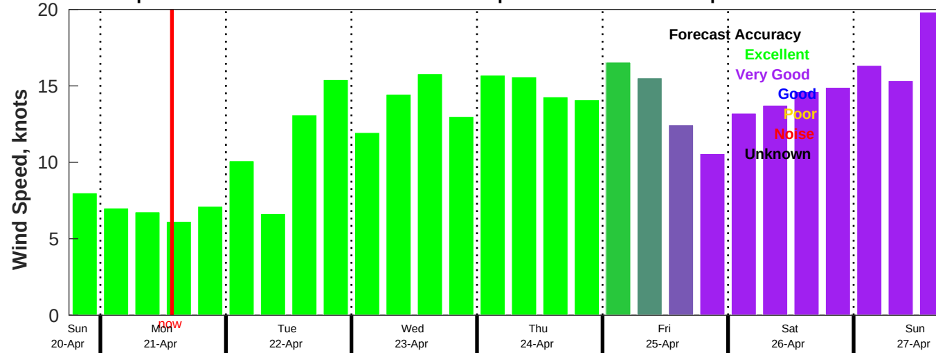
AUSWAV Wind Speed Forecast for NDBC 42020 from 20-Apr-2025 18:00:00 to 27-Apr-2025 18:00:00
