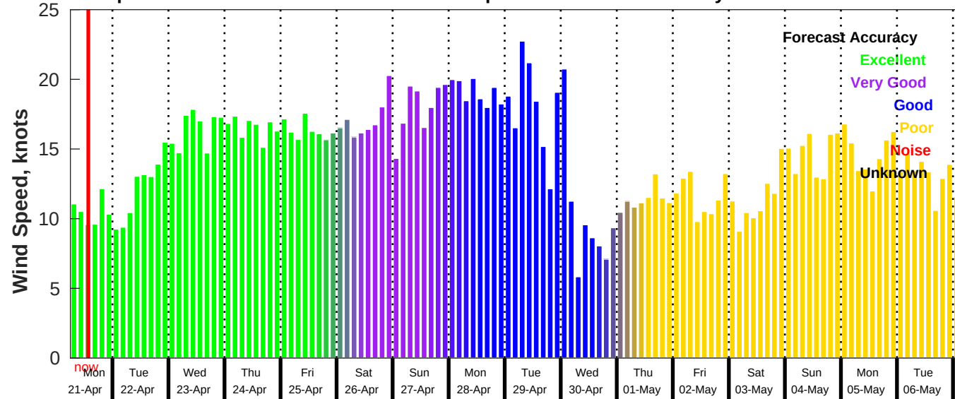
GFS Wind Speed Forecast for NDBC 42020 from 21-Apr-2025 06:00:00 to 07-May-2025 06:00:00
