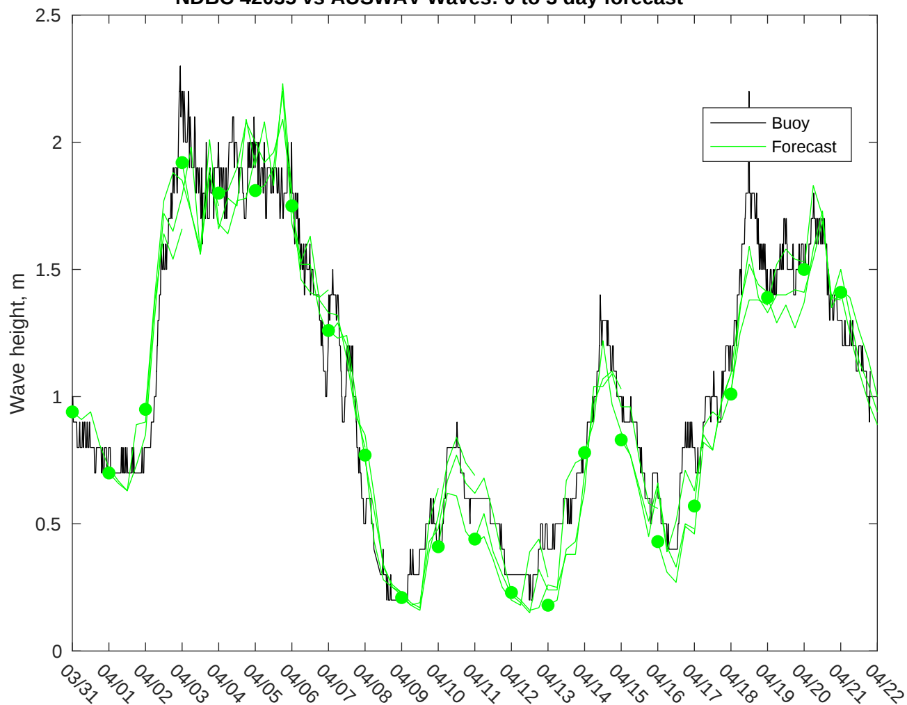
NDBC 42035 vs AUSWAV Waves: 0 to 3 day forecast
