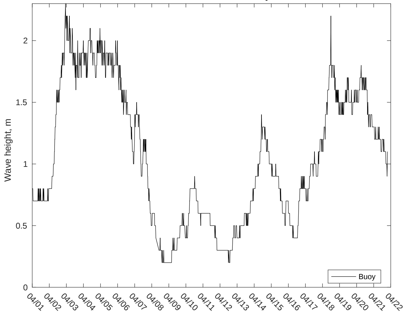
NDBC 42035 vs AUSWAV Waves: 10 to 16 day forecast
