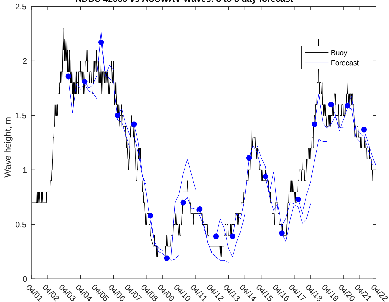
NDBC 42035 vs AUSWAV Waves: 3 to 5 day forecast
