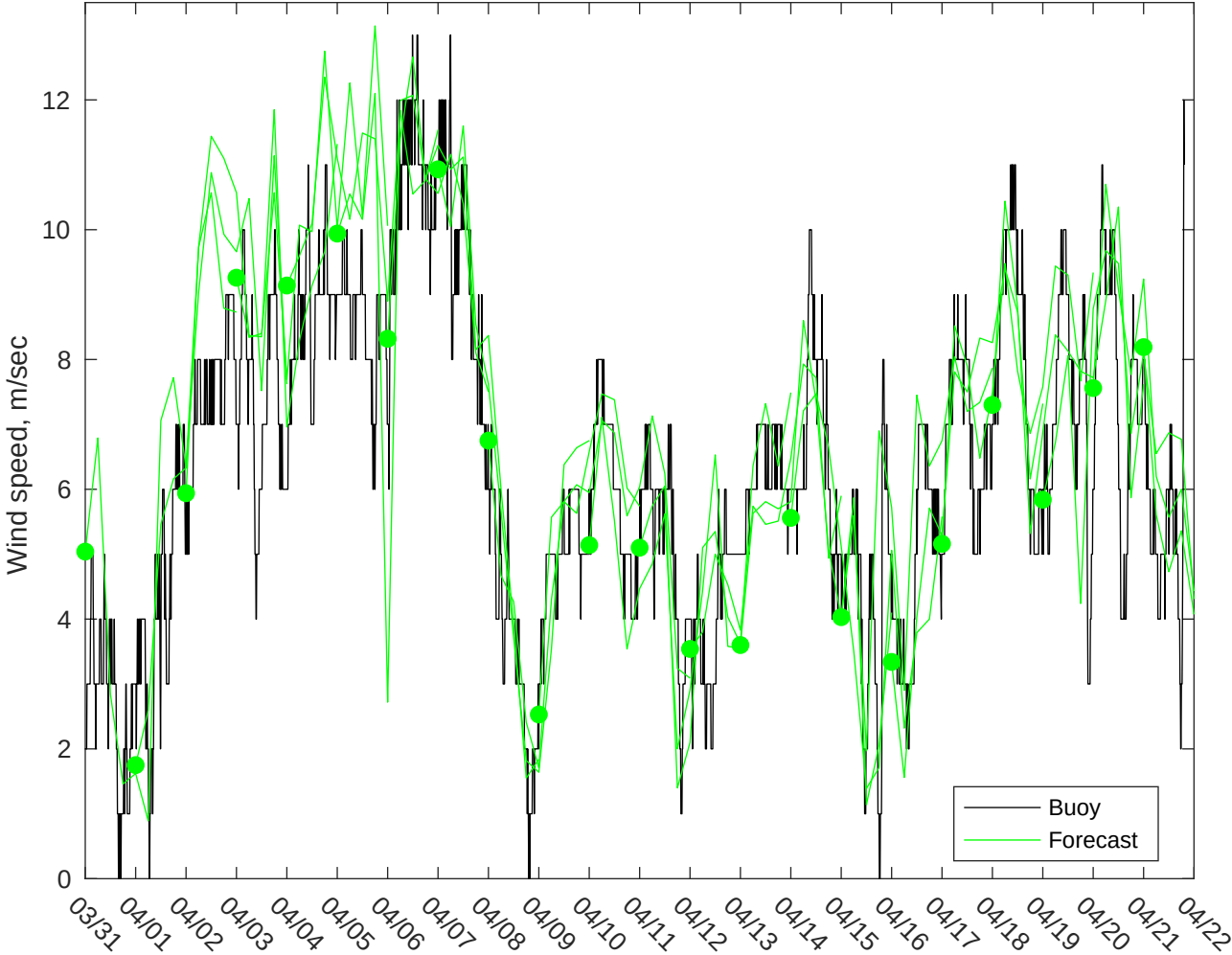
NDBC 42035 vs AUSWAV Winds: 0 to 3 day forecast
