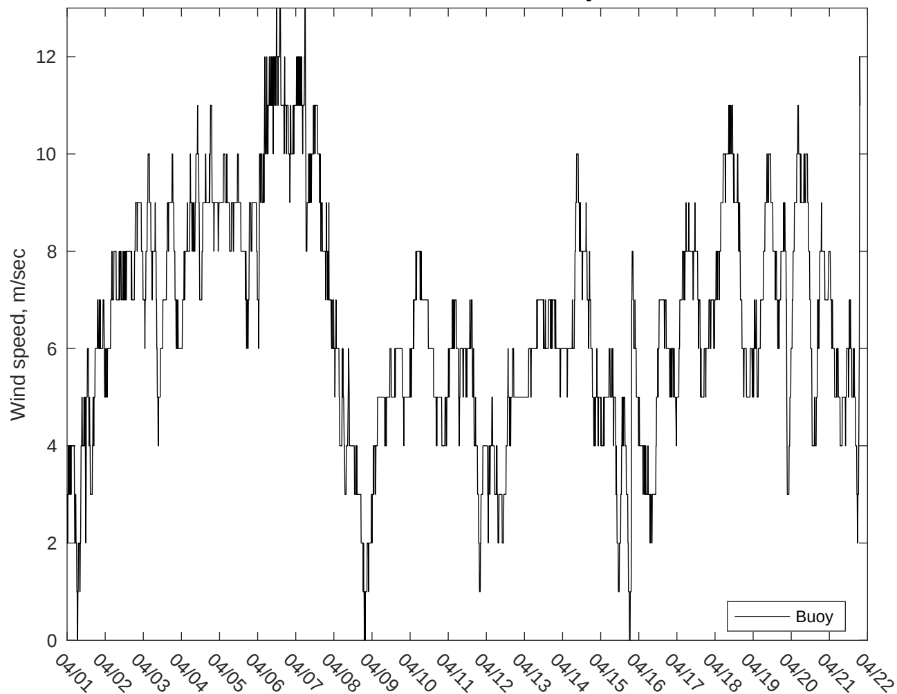
NDBC 42035 vs AUSWAV Winds: 10 to 16 day forecast
