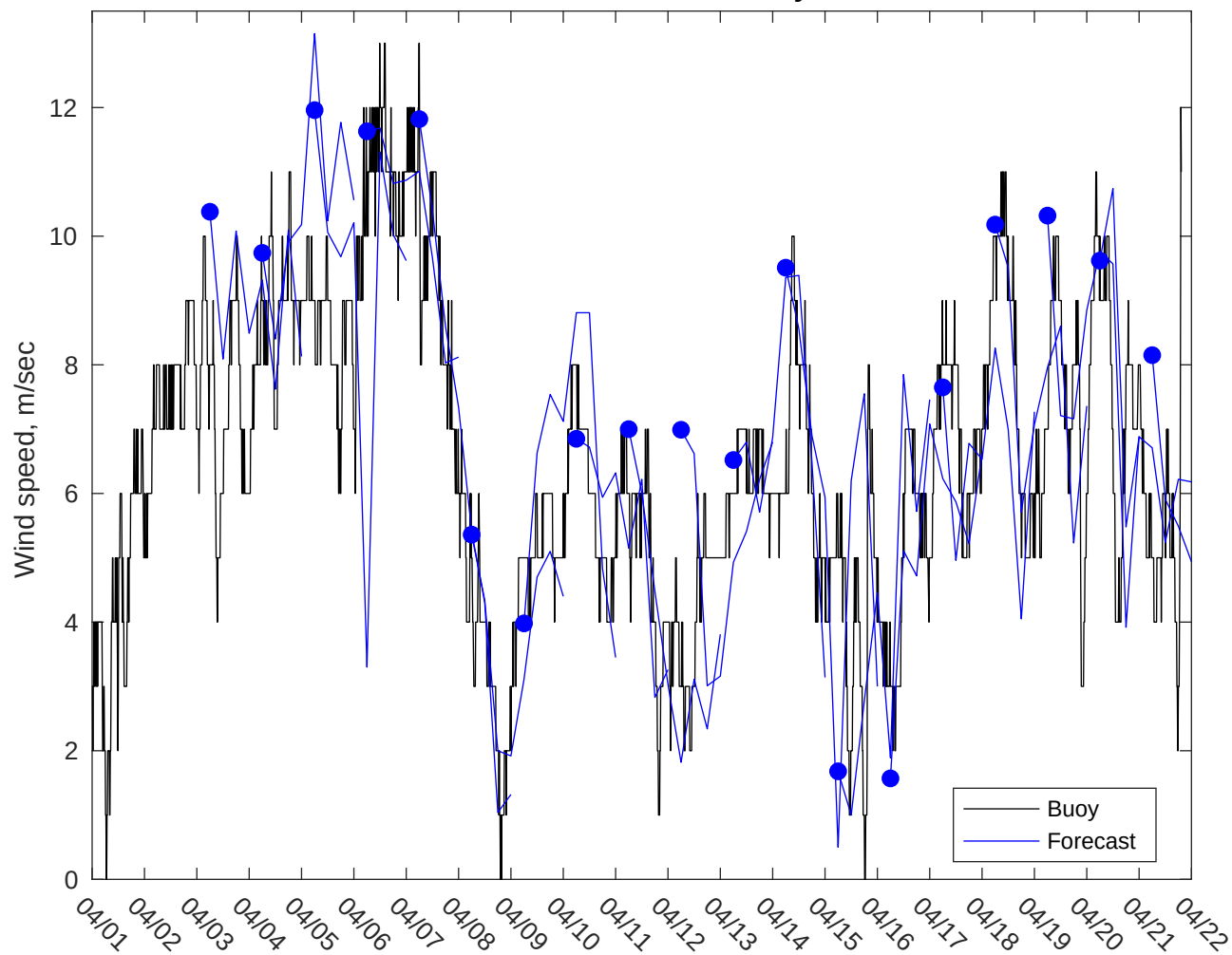
NDBC 42035 vs AUSWAV Winds: 3 to 5 day forecast
