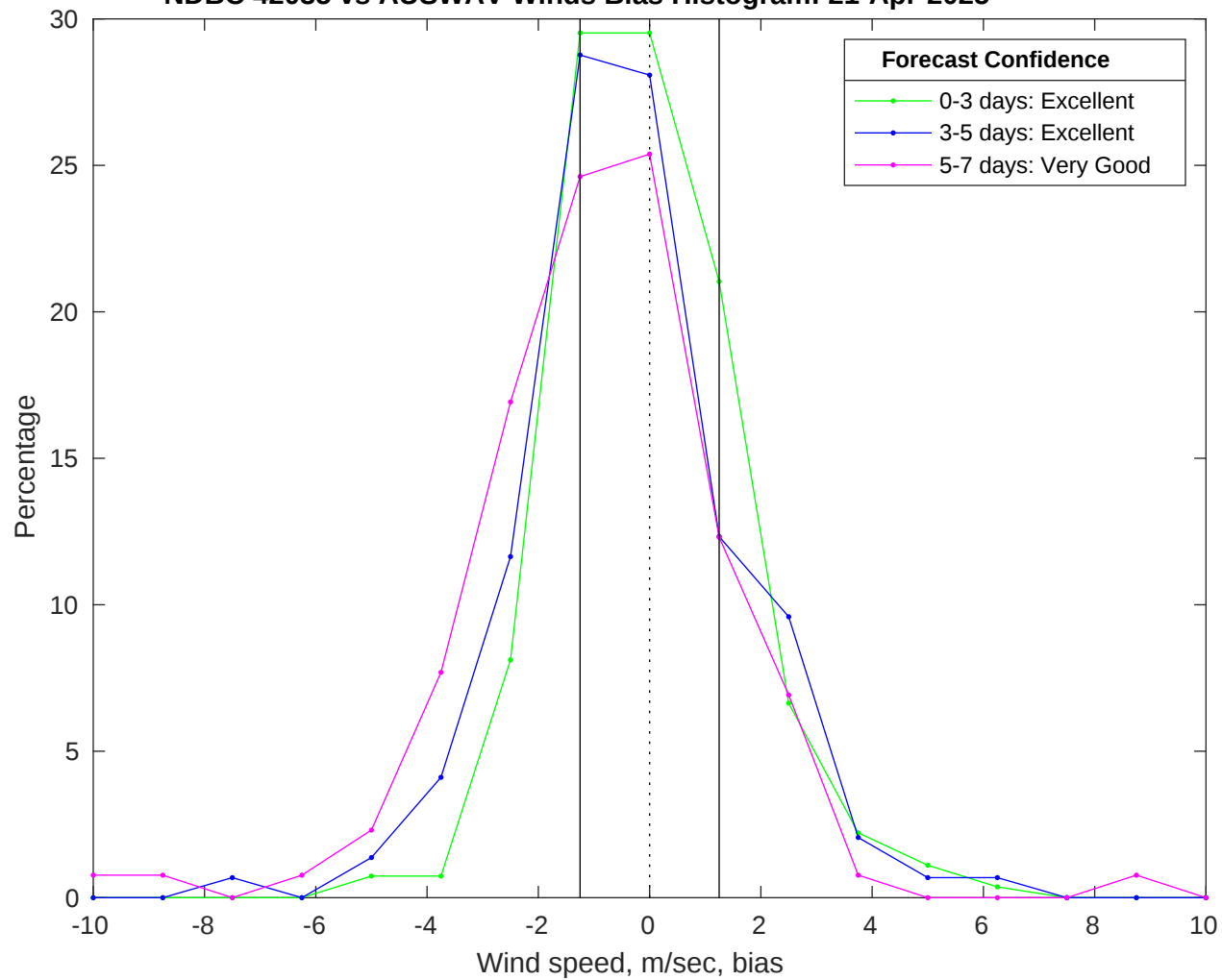
NDBC 42035 vs AUSWAV Winds Bias Histogram: 21-Apr-2025
