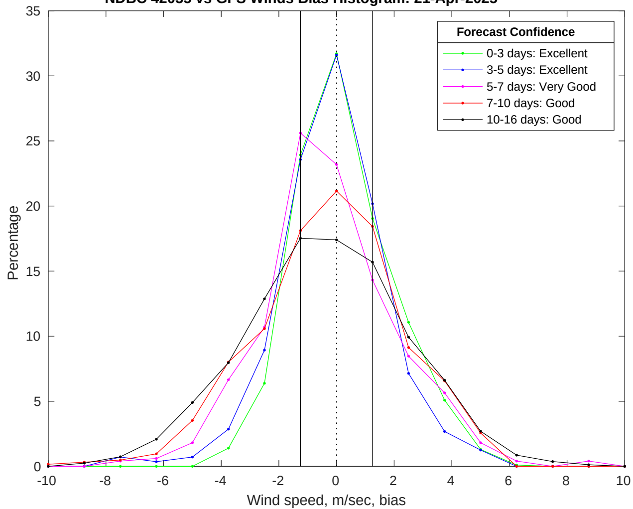
NDBC 42035 vs GFS Winds Bias Histogram: 21-Apr-2025
