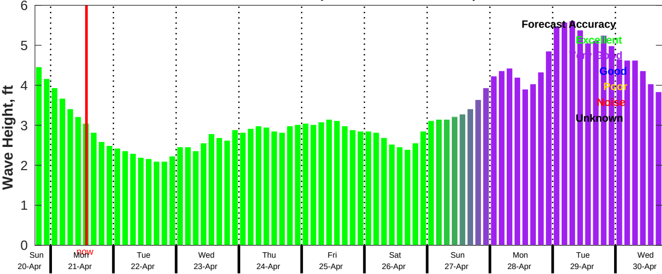
CMEMS Wave Forecast for NDBC 42035 from 20-Apr-2025 18:00:00 to 30-Apr-2025 18:00:00
