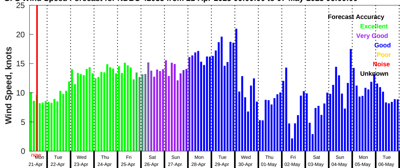
GFS Wind Speed Forecast for NDBC 42035 from 21-Apr-2025 06:00:00 to 07-May-2025 06:00:00
