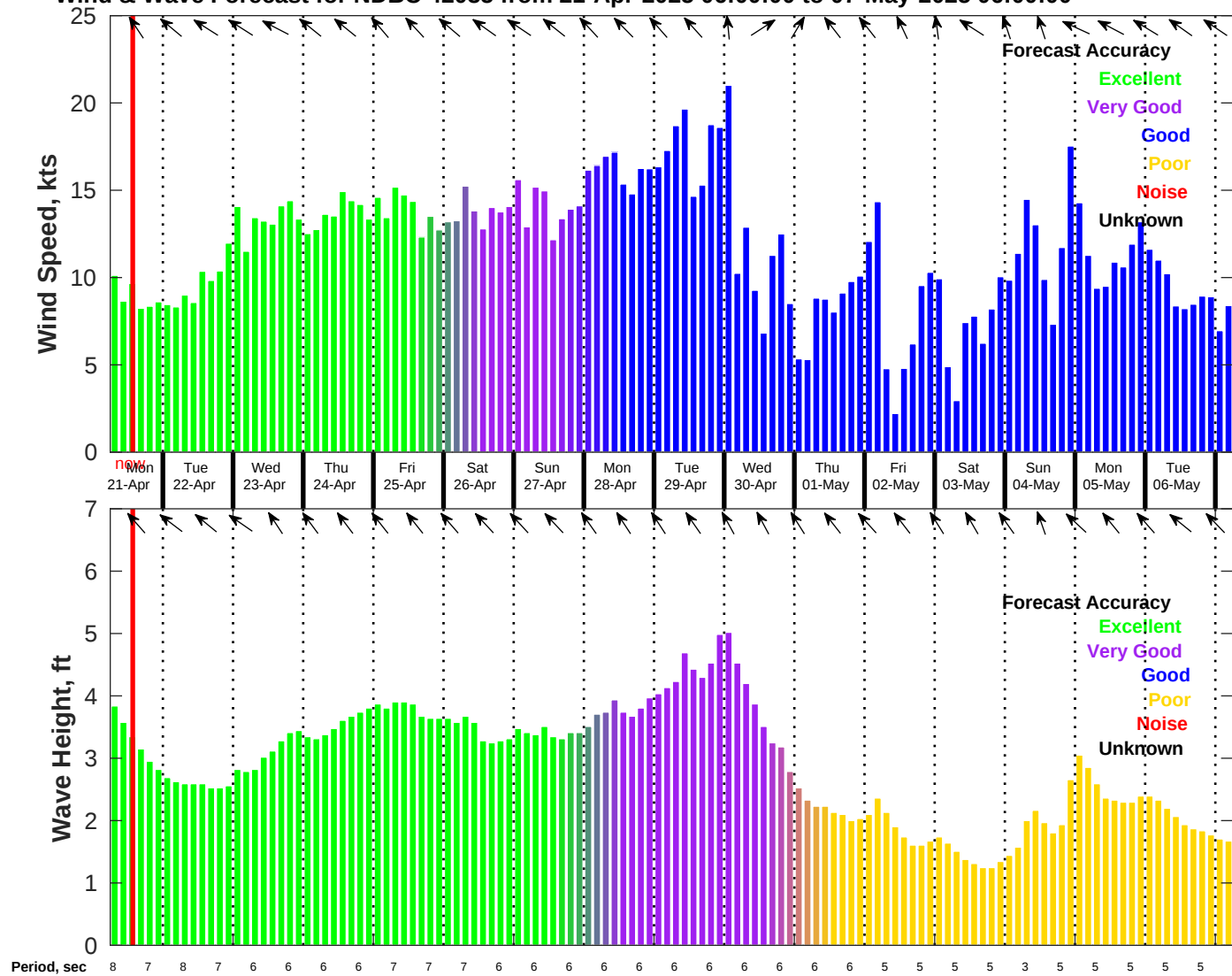
Wind & Wave Forecast for NDBC 42035 from 21-Apr-2025 06:00:00 to 07-May-2025 06:00:00
