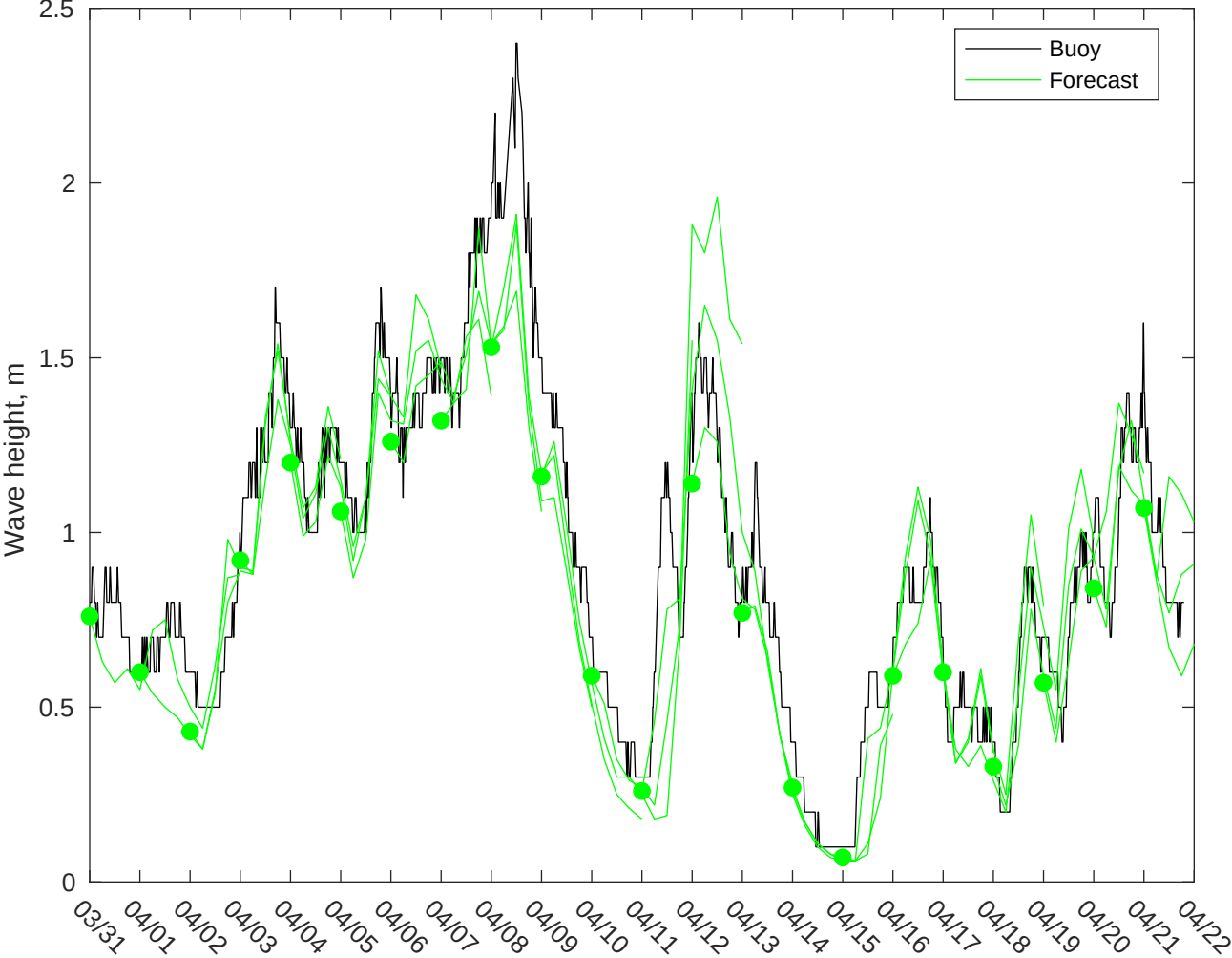
NDBC 42036 vs AUSWAV Waves: 0 to 3 day forecast
