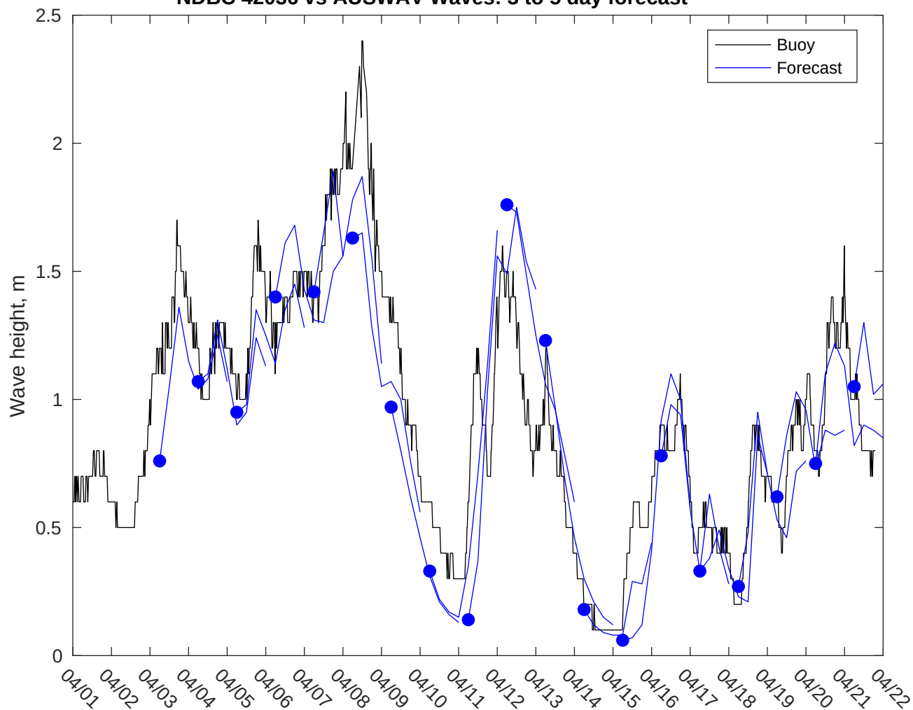
NDBC 42036 vs AUSWAV Waves: 3 to 5 day forecast
