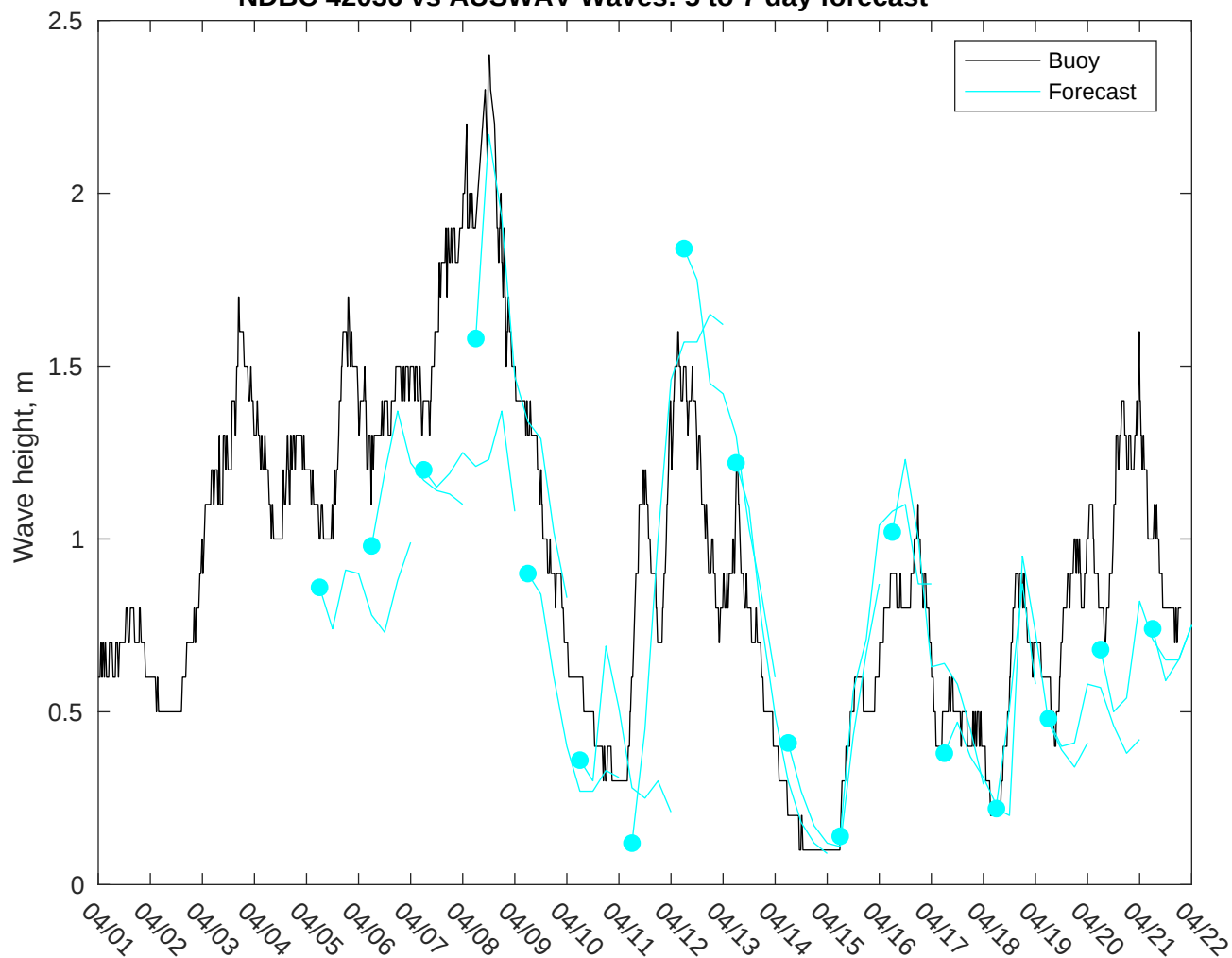
NDBC 42036 vs AUSWAV Waves: 5 to 7 day forecast
