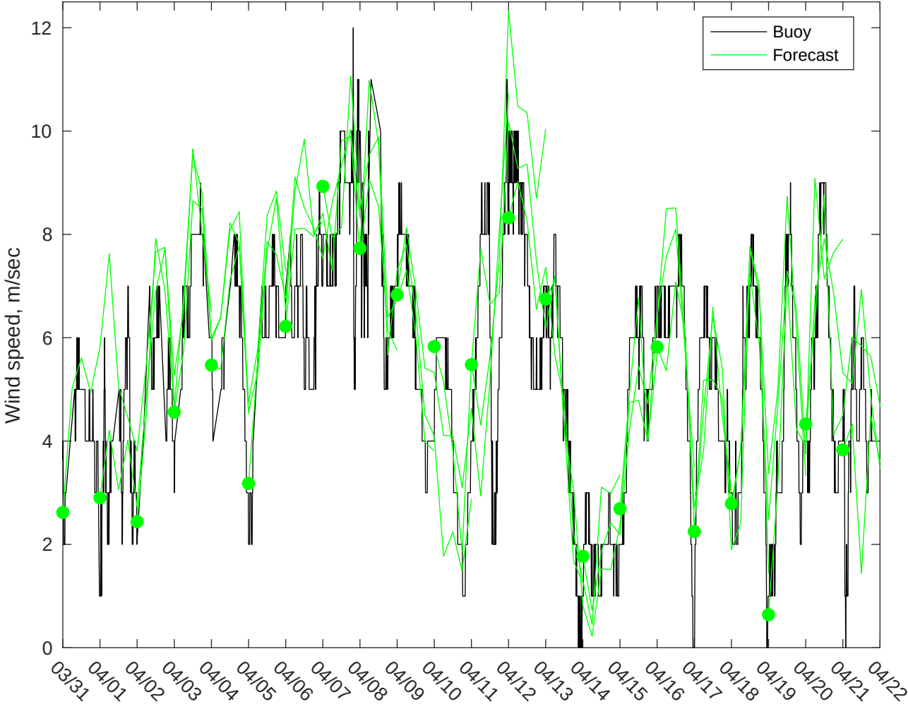
NDBC 42036 vs AUSWAV Winds: 0 to 3 day forecast
